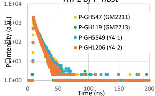
TRPL of P-host
