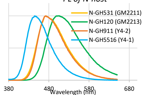
PL of N-host
