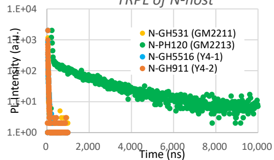
TRPL of N-host
